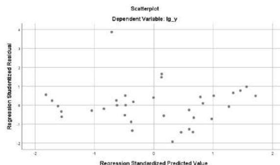
Figure 4.1 Heteroscedasticity Test
